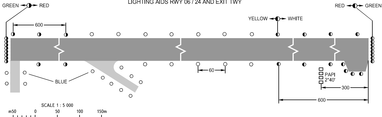
LIGHTING AIDS RWY 06 / 24 AND EXIT TWY
