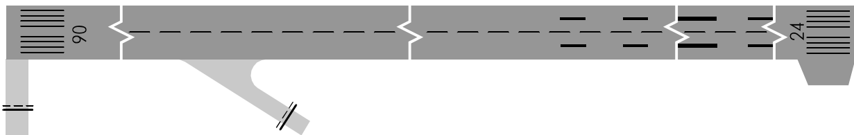
LIGHTING AIDS RWY 06 / 24 AND EXIT TWY
